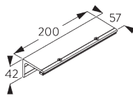
SG 6503 Bracket
